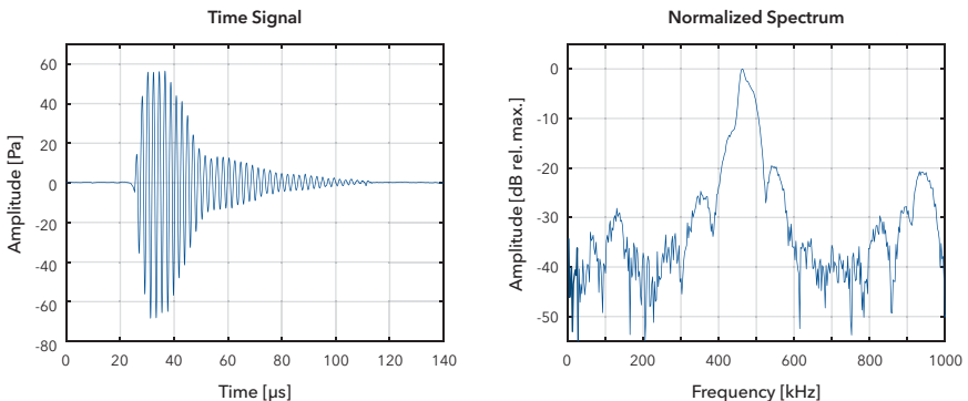
Time signal and normalized spectrum of a piezoelectric emitter measured with the optical microphone
