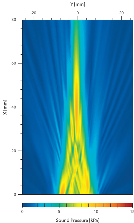
Ultrasound field scan of a piezoelectric emitter with an optical microphone
